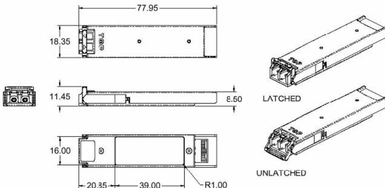
XFP Transceiver (dimensions are in mm)
